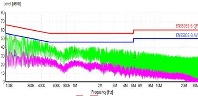
Conduction EMI--LINE
