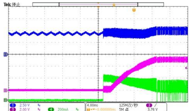
Over Temperature Protection Recovery (CH1-VDD, CH2-VO, CH4-IL)
