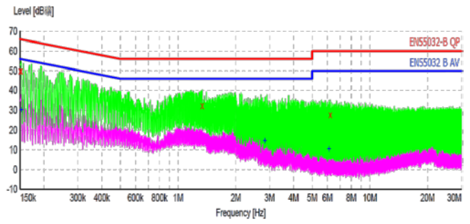
Conduction EMI--NEUTRAL
