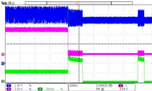
Short Load Protection (CH1-VDD, CH2-VO, CH4-IL)
