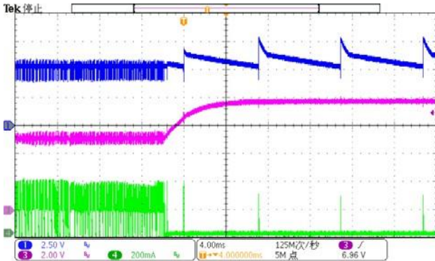
Over Voltage Protection (CH1-VDD, CH2-VO, CH4-IL)
