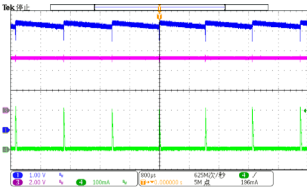
system Steady State(No Load) (CH1-VDD, CH2-VO, CH4-IL)
