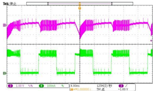
Load Transient(50mA-200mA, 0.5A/us) (CH2-Vo ripple, CH4-Io)
