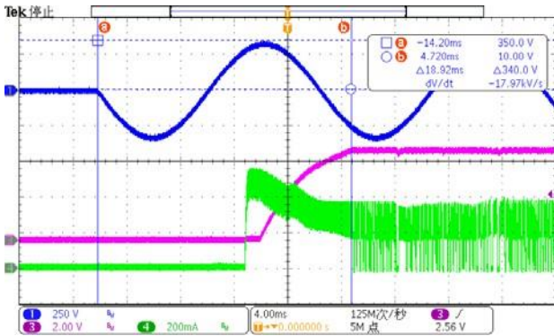
System Startup Time (CH1-VINAC, CH2-VO, CH4-IL)
