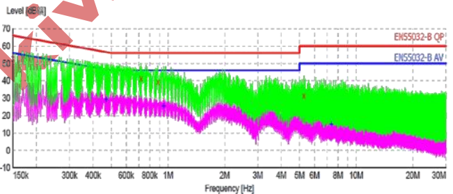
Conduction EMI--LINE
