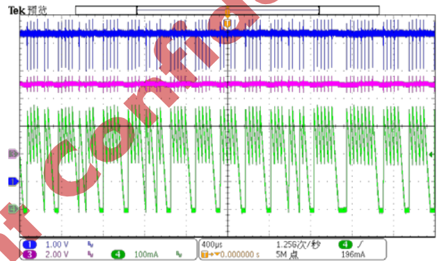
System Steady State(Full Load) (CH1-VDD, CH2-VO, CH4-IL)
