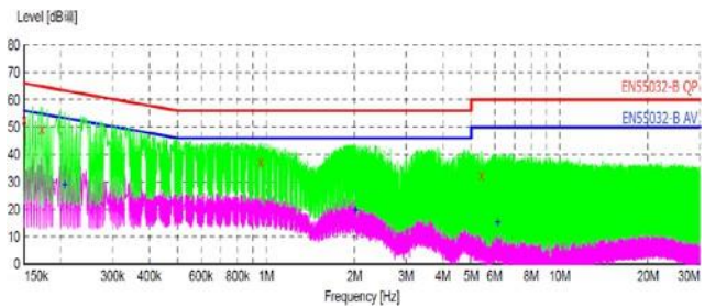
Conduction EMI--NEUTRAL
